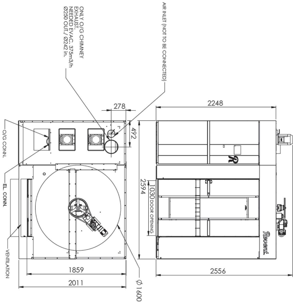
REVENT RACK OVEN 723 701141
